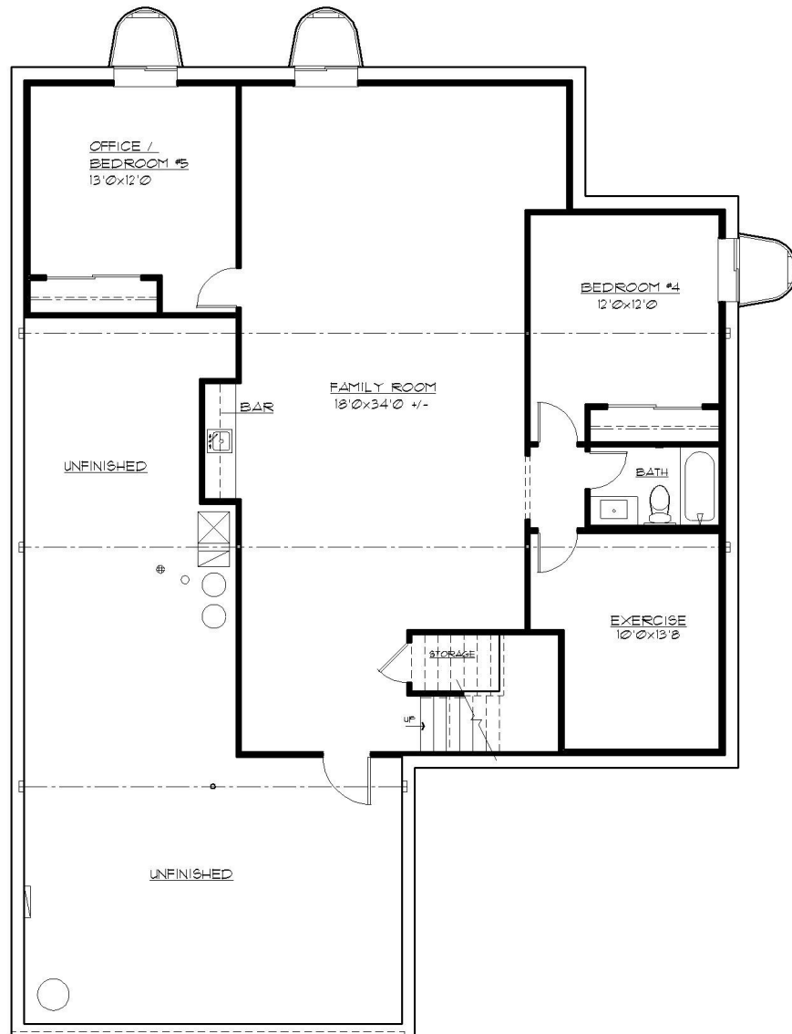
LOWER LEVEL PLAN 1,409 SQ. FT.
