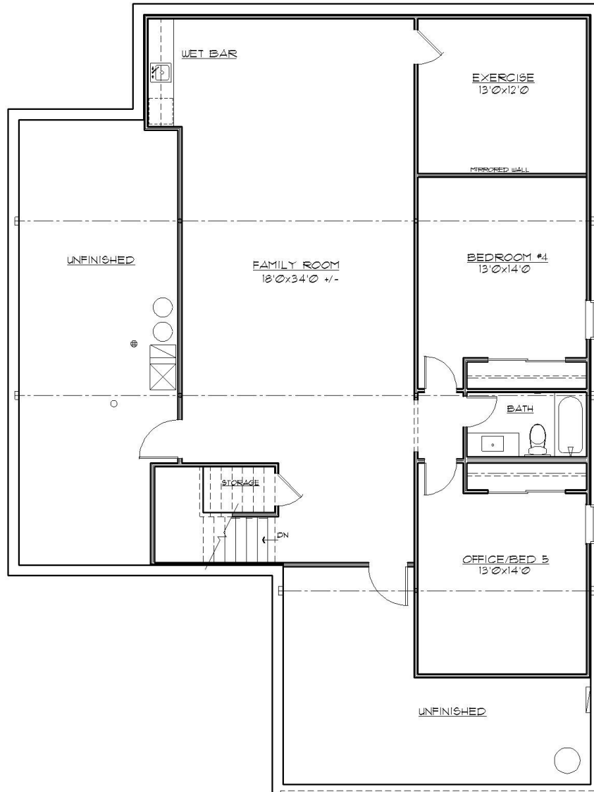
LOWER LEVEL PLAN 1,414 SQ. FT.
